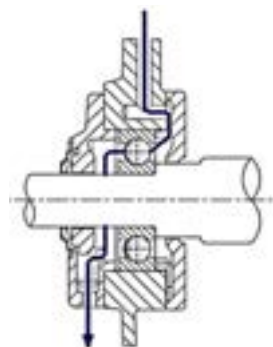
GREASE PATH
